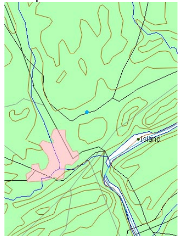
map scale 1:200,000
