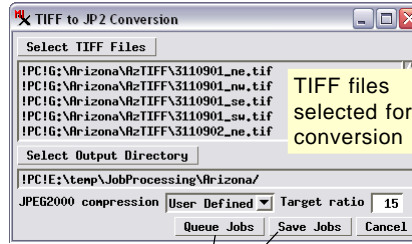
Procedure to make job files in I/O script TiffToJP2getJobParms.sml (further excerpts on reverse of this page)
