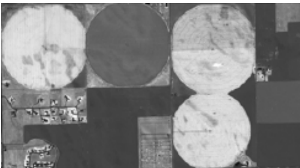
G Rand U nified V egetation Index (GRUVI) image of the fields computed by the GRUVI script using an optional background soil adjustment parameter optimized for this image. Soil surface wetness variations are not visible and do not contaminate the biomass signal in this image.
