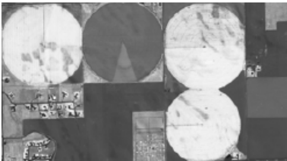
Traditional N ormalized D ifference V egetation Index (NDVI) image of the fields computed using optional settings in the GRUVI script. Higher NDVI (brighter tones) are meant to indicate higher vegetation biomass, but NDVI is also unduly influenced by background soil surface wetness; note the wedge of wet soil in the top center circular field is obvious and appears brighter than the adjacent dry soil background.
