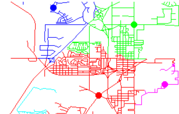
Streets allocated to different distribution centers (circles)
